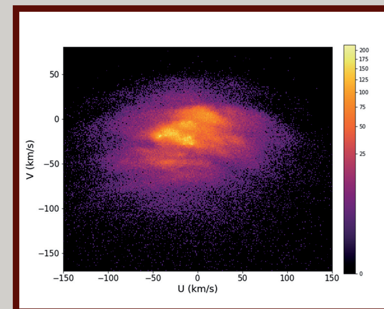
2018 (Gaia) 366 238 stars
